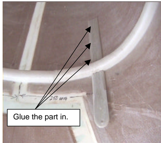
Cut seat belt attachment # 2-1061 in two pieces and fare them out on both sides and on the ends to glass them easy in.
